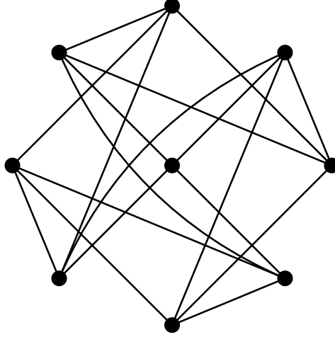
Figure 1 A self-complementary vertex transitive graph on 9 vertices.
