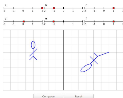
Figure 14.4. Affine Transformations
