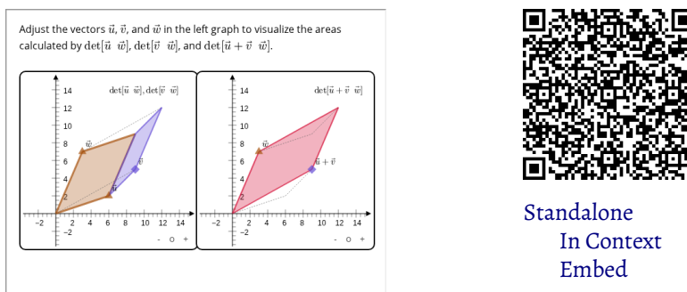
Figure 14.34. DoenetML example
