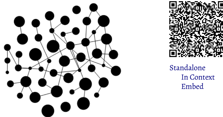
Figure 14.9. Graph Layout
