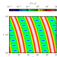
Figure 27.9(b). Asymptote Contour Plot
