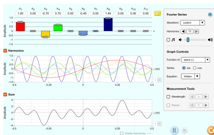
Figure 15.6. Fourier: Making Waves iframe
