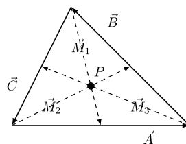
Figure 37.3. The medians of the triangle are \vec{M}_1 , \vec{M}_2 , and \vec{M}_3 .
