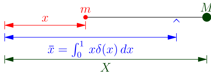
Figure 10.19. Asymptote Lever, plus Integral
