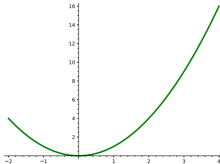
Figure 10.27. A Sage standard parabola, on [-2, 4]
