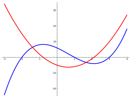
Figure 5.2. A function and its derivative
