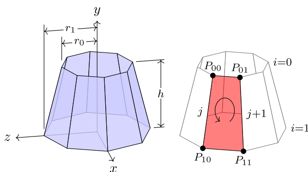
Figure 10.8. TikZ Cone Drawing
