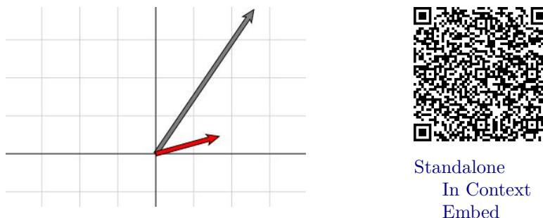
Figure 14.1. A simple eigenvector demonstration
