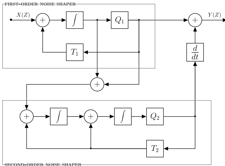
Figure 10.7. TikZ Electronics Diagram
