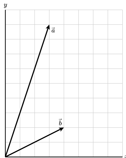
Figure 37.19. Two vectors \vec{a} and \vec{b} .
