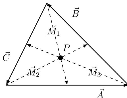
Figure 37.8. The medians of the triangle are \vec{M}_1 , \vec{M}_2 , and \vec{M}_3 .
