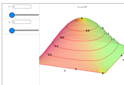
Figure 15.4. Probability wavefunction with contours (includes controls)
