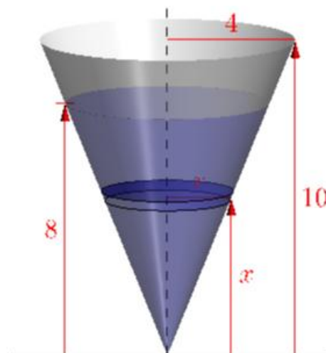
Figure 10.20. Work Cone (Asymptote Interactive 3D Image)
