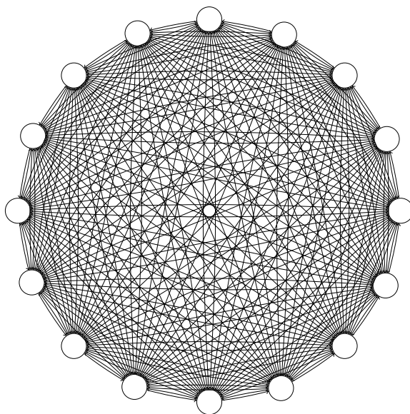
Figure 10.3. Complete graph on 16 vertices, from www.texample.net
