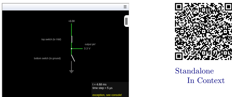
Figure 15.10. CircuitJS with resize-behavior="responsive"
