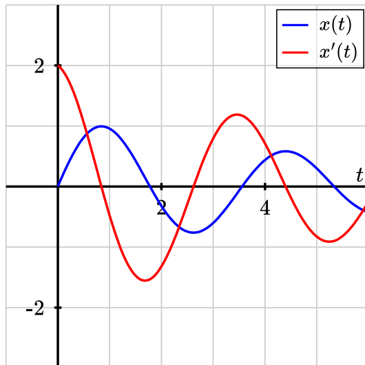
Figure 10.5. Solution to a differential equation
