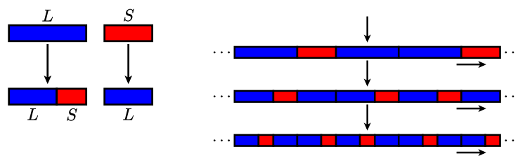
Figure 10.6. Fibonacci tilings are one-dimensional analogs of Penrose tilings. The diagram on the left introduces the process of deflation that is used to produce tilings while the diagram on the right explains why they are aperiodic.
