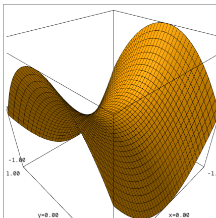
Figure 14.33. threejs saddle by Sage
