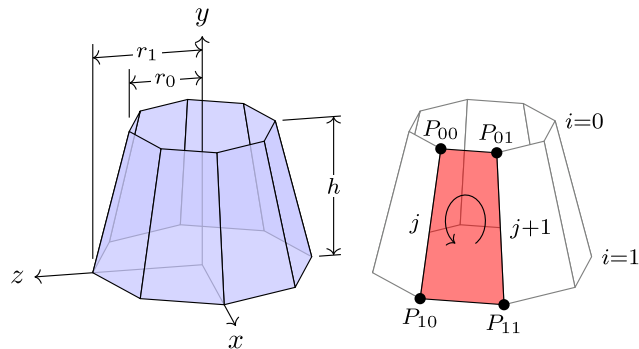
Figure 10.7. TikZ Cone Drawing
