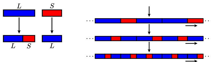
Figure 10.5. Fibonacci tilings are one-dimensional analogs of Penrose tilings. The diagram on the left introduces the process of deflation that is used to produce tilings while the diagram on the right explains why they are aperiodic.
