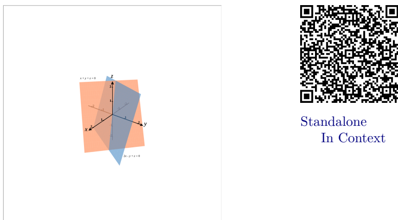
Figure 15.3. Intersection of two planes (minimal embedding)
