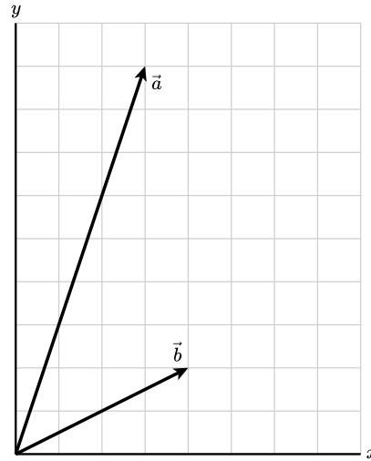
Figure 37.19. Two vectors \vec{a} and \vec{b} .
