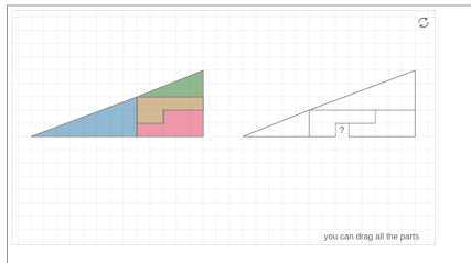
Figure 15.1. Right Triangle Paradox
