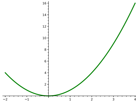
Figure 10.23. A Sage standard parabola, on [-2, 4]
