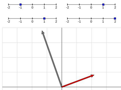
Figure 14.3. Eigenvector demonstration
