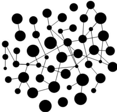
Figure 14.9. Graph Layout
