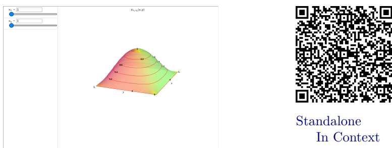
Figure 15.4. Probability wavefunction with contours (includes controls)
